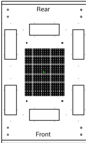
Top Panel 600W x 1000D
