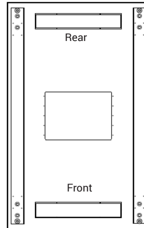
Bottom Panel 600W x 1000D
