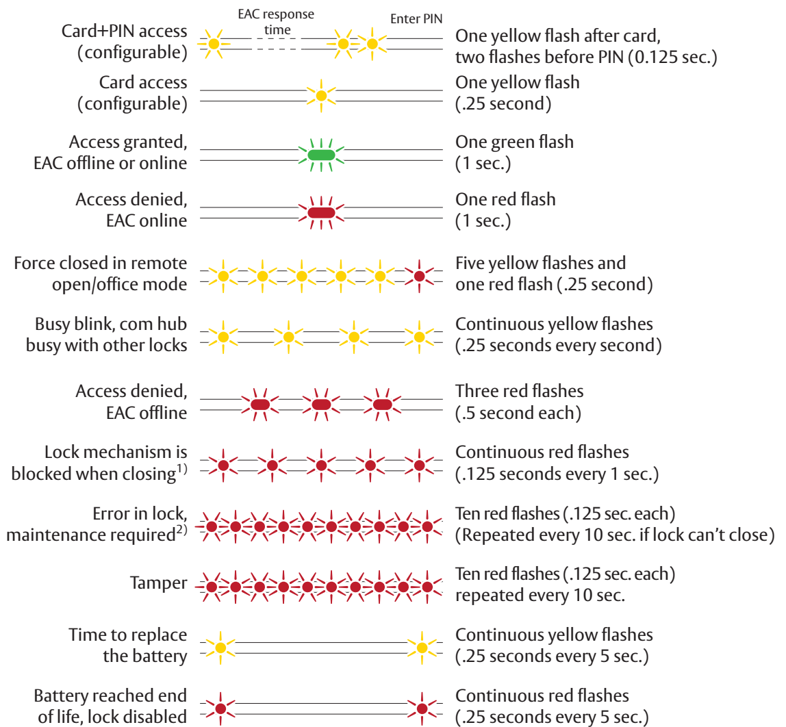
Figure 5. Lock normal operation LED indication
