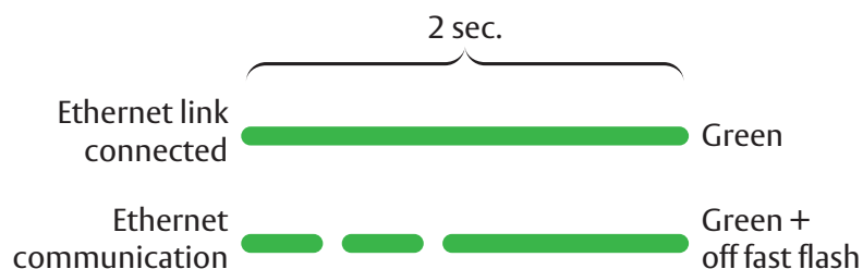
Figure 4. AH40 Communication hub Ethernet LED indication
