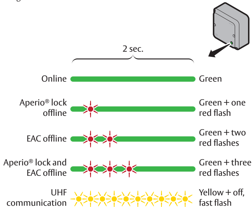
Figure 2. Communication hub normal operation LED indication
